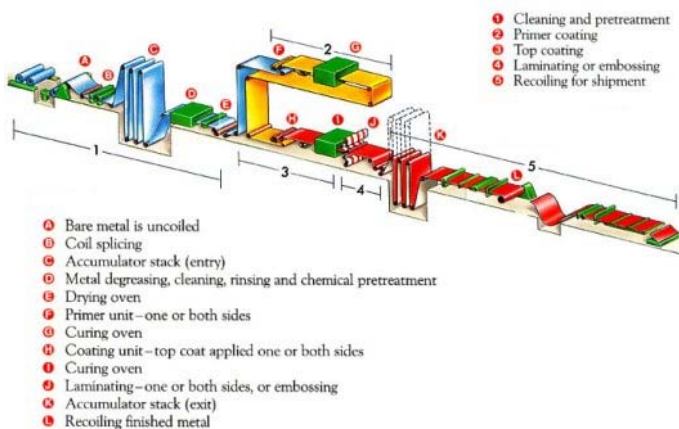
Step 2 Painting Process 40 Yr. Paint Warranty
